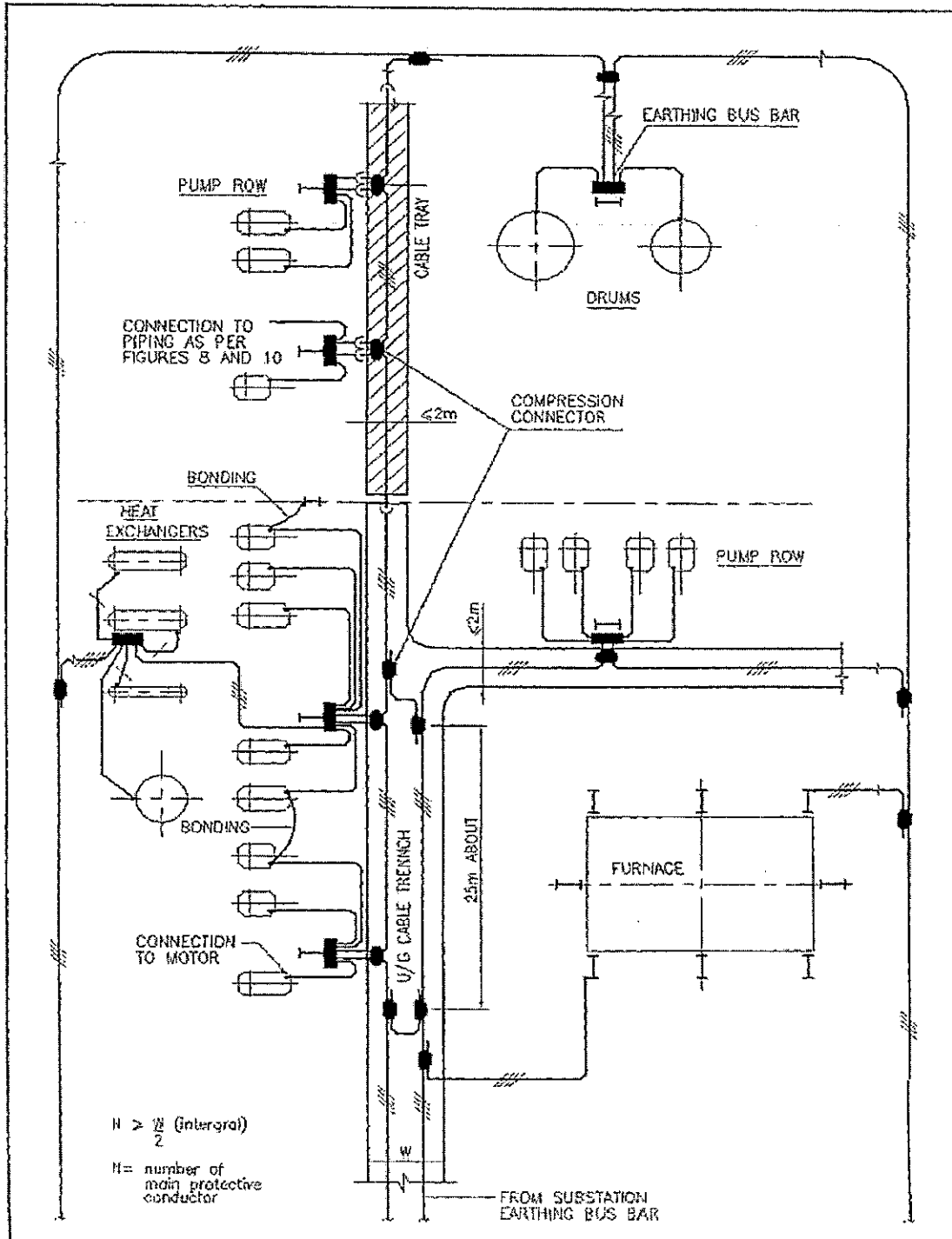
FIGURE 1 TYPICAL EARTHING NETWORK LAYOUT
