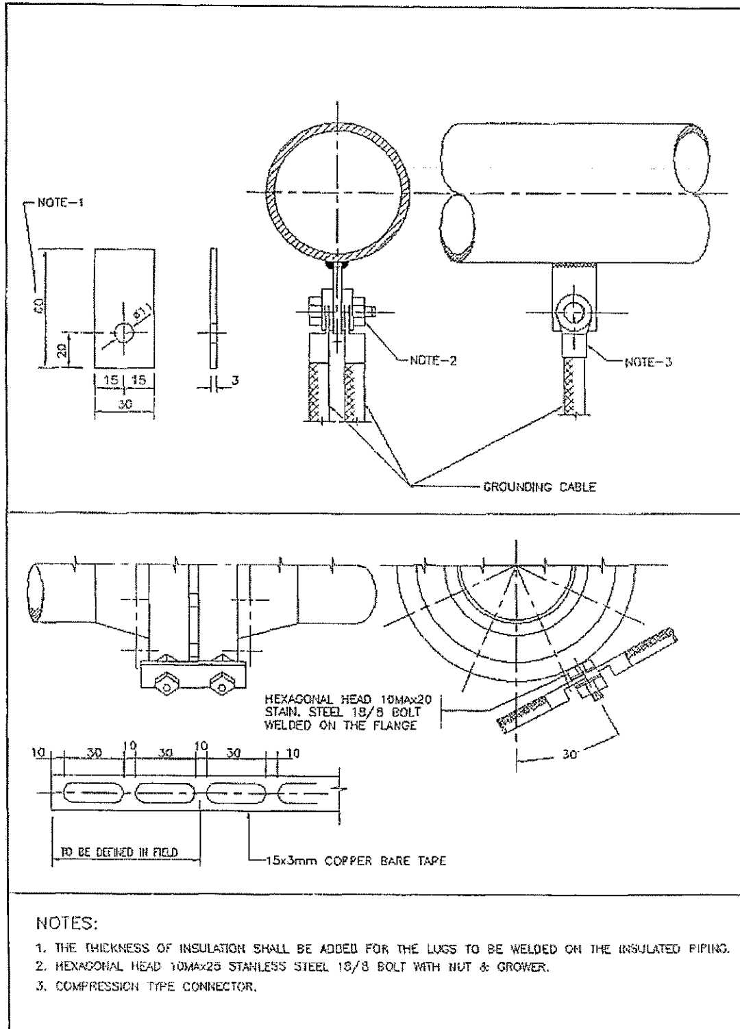
FIGURE 9 TYPICAL JUMPER DETAILS
